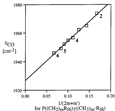
Figure 2. Relationship between IR \nu_{\text{CO}} values of 15–22 , and the reciprocal of the total number of methylene groups in each phosphane ligand; selected ligands are designated by numbers for reference
